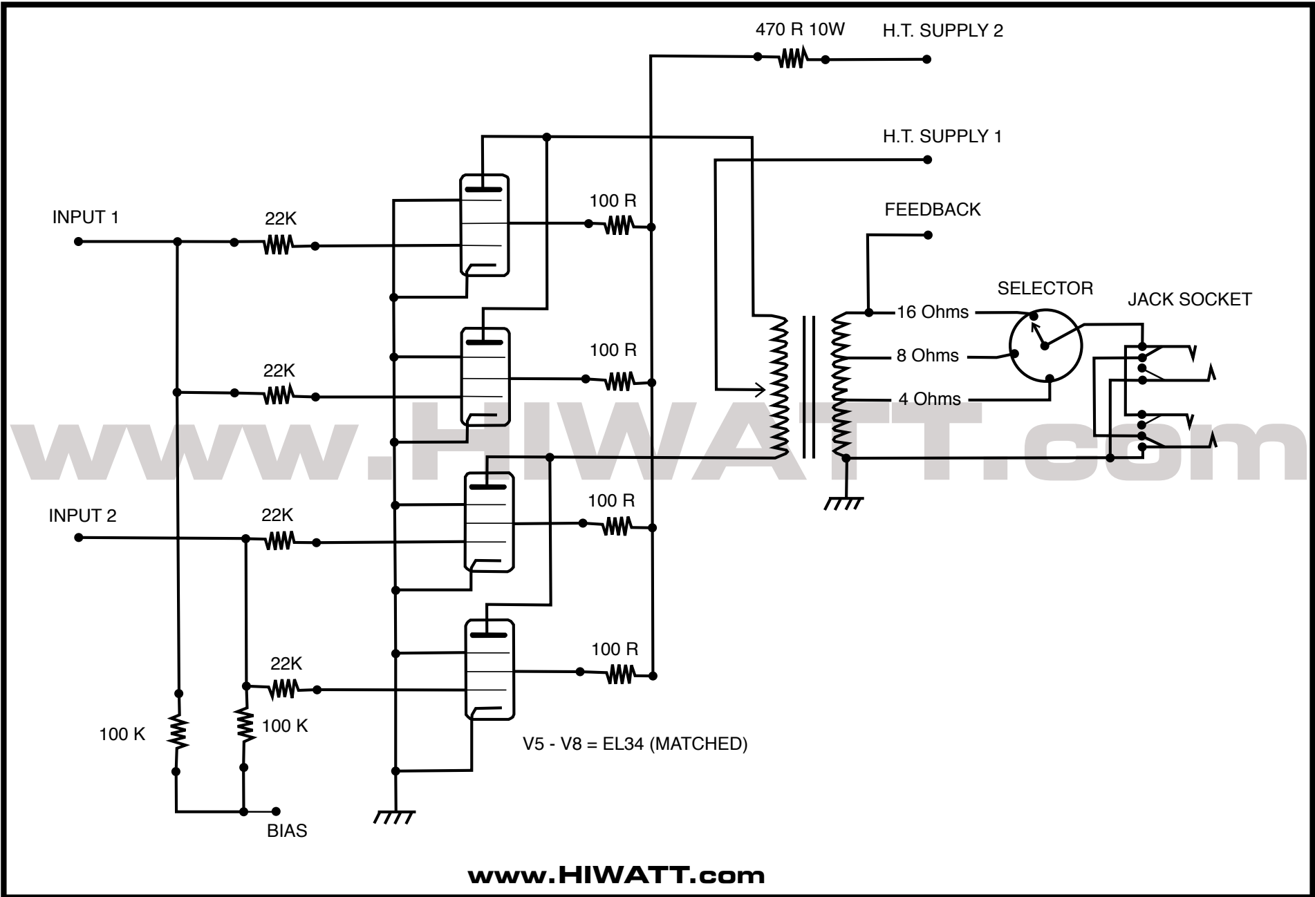
HIWATT® DR103 OUTPUT STAGE CIRCUIT DIAGRAM Copyright © HIWATT Amplification 2001
